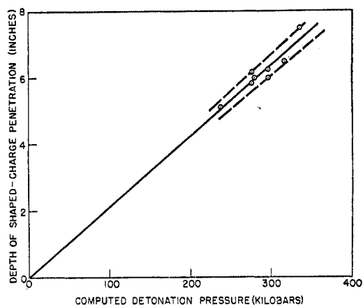
Fig. 1. Shaped-charge effect as a function of detonation pressure
